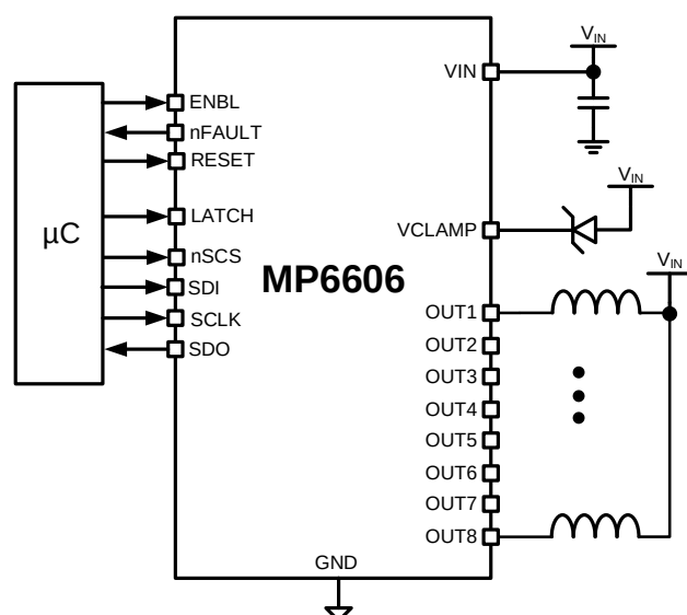
Figure 6: Typical Application Circuit
