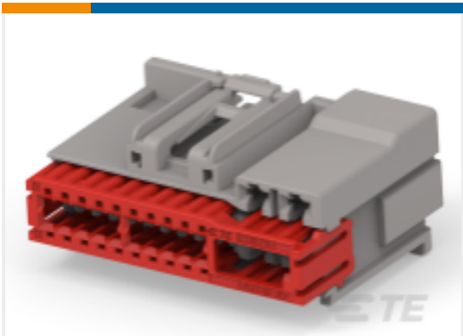
TE Part # 1-2236269-1 24POS, MIXED,REC HSG, 20GENYMCP,ASSY,CODA
