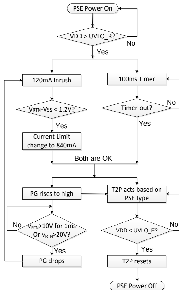
Figure 3: Start-Up Sequence
