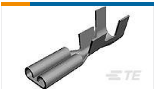
TE Part # 170213-1 250 FASTON,REC.,18-14 AWG,BR
