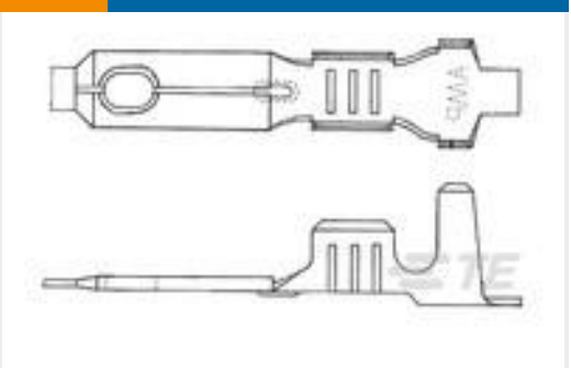
TE Part # 880633-1 110 FASTON REC 20-17 AWG BR
