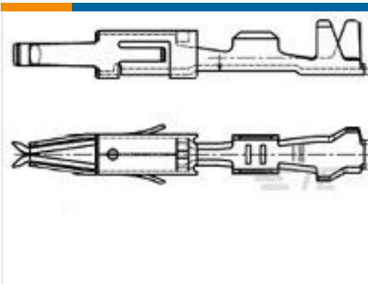
TE Part # 1241844-2 MT2 A REC 1.6 Contact SRC Sn
