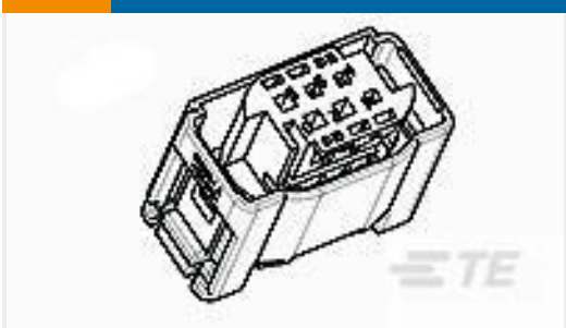
TE Part # 1-967616-2 6POS MQS REC SEALED COD A
