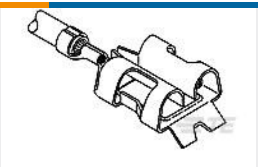
TE Part # 640748-7 HEAVY DUTY BURNER REC 18-14 AWG PHBRZ
