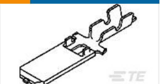
TE Part # 170340-3 FF 250 TAB 20-14AWG PTBR WITHOUT LATCH
