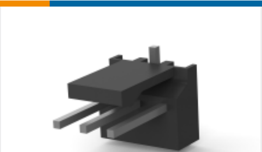
TE Part # 2232980-3 03P MTA100 HDR ASSY SM 30AU W
