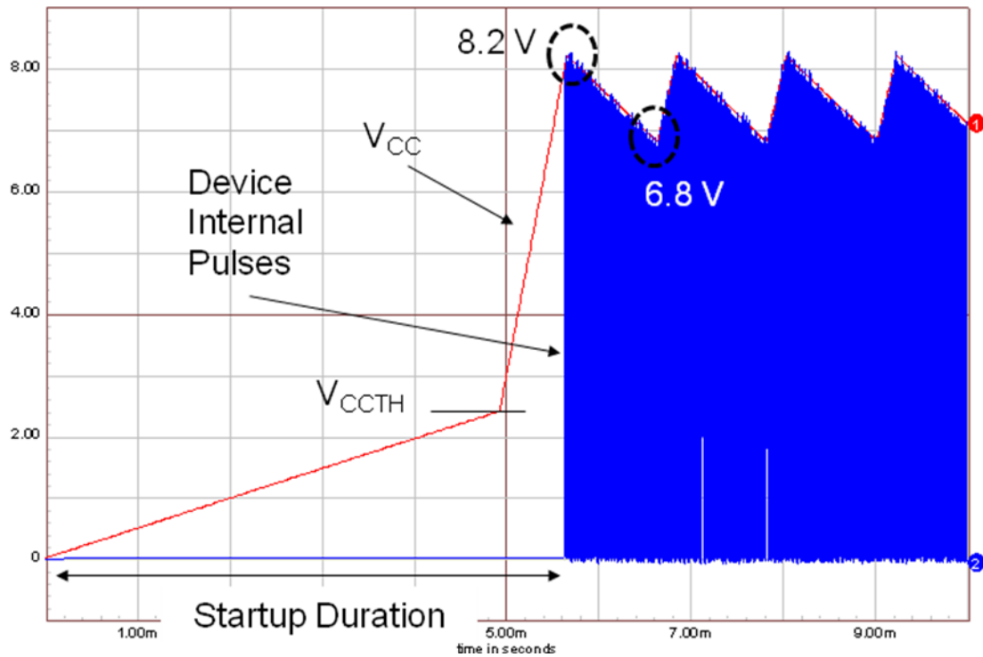
Figure 25. The Charge/Discharge Cycle Over a 1 \mu\text{F} V_{\text{CC}} Capacitor
