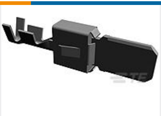
TE Part # 964306-1 TAB A 5.8x0.8 CONTACT CF SRC Sn
