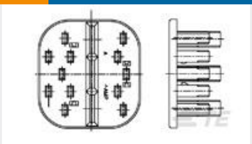
TE Part # 85223-1 E-J MK-II(+) 15P PLUG DBL
