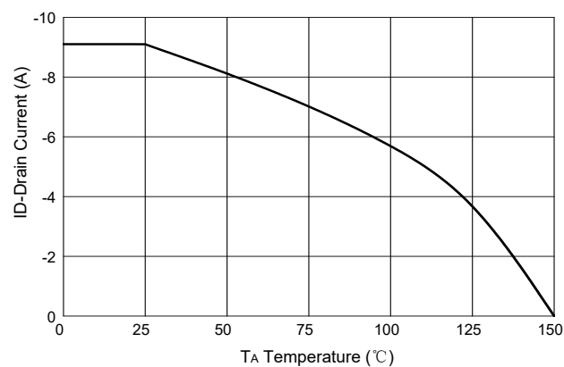
Fig.10 - Drain Current
