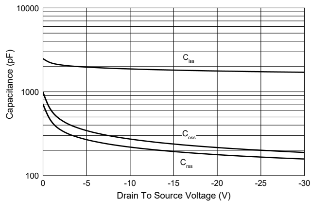
Fig.5 - Capacitance Characteristics
