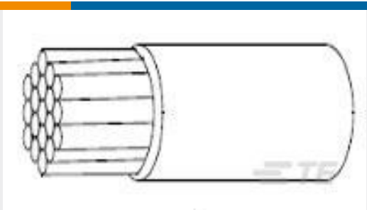
TE Part # 156160-001 22759/32-22-1
