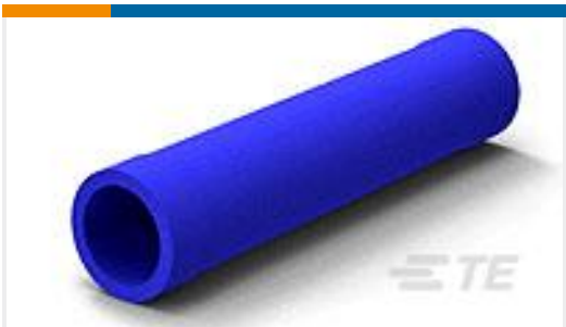
TE Part # 2-34071-1 SPLICE,PG BUTT 16-14,STRAIGHT
