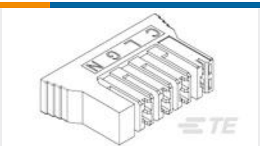
TE Part # 521781-1 250 HSG. PL MKIII REC. 6.81mm 4P NAT
