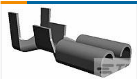
TE Part # 62181-1 187 FASTON REC 24-20 AWG TPBR
