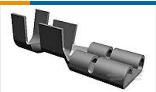
TE Part # 280000-6 250 FASTON,REC.,24-17 AWG,TPBR
