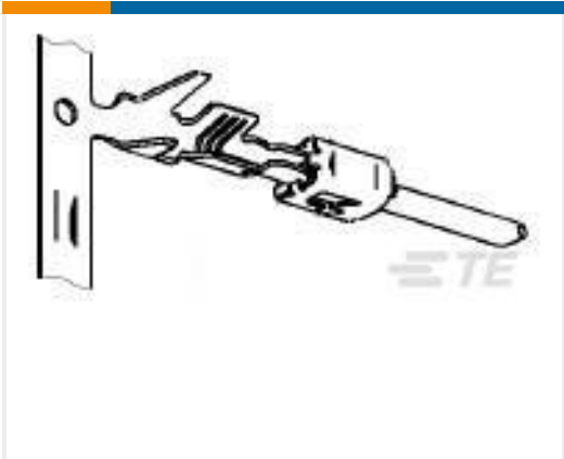
TE Part # 2-2141598-2 TAB 2.8x0.8 CONTACT CF SRC Ag
