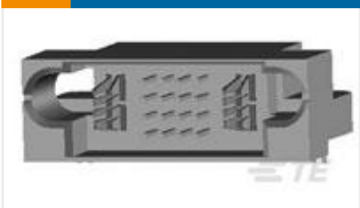
TE Part # 8-6450130-5 MBXL R/A HDR 1P+16S+1P
