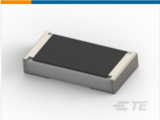
TE Part # 2176468-6 TLRP 2010 1.0W R075 1% 75PPM 4K RL
