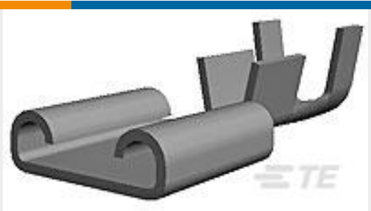
TE Part # 170187-2 250 FASTON, REC., 22-18 AWG, TPBR
