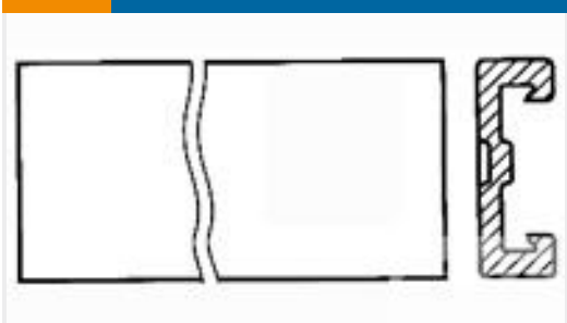
TE Part # 640642-6 06P MTA100 COVER F/T
