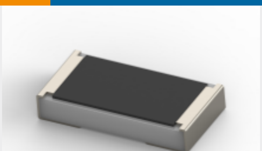
TE Part # 1-2176232-4 SMD Power Resistor: 3 Watt, 1% Tol
