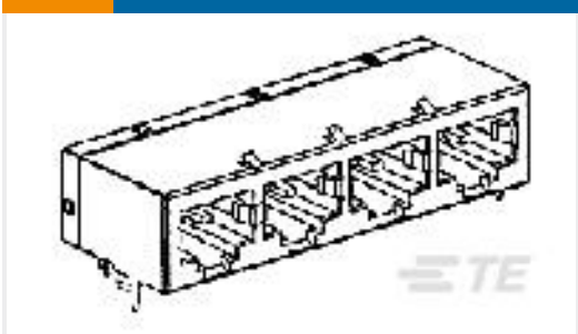
TE Part # 5558503-1 MJ ASSY,4P,8 POS,CAT 5E,PCB GND
