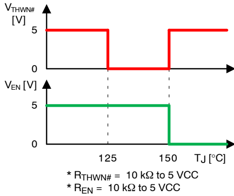
Figure 38. V_{THWN\#} , V_{EN} vs. Driver Temperature
