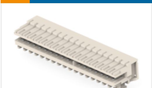
TE Part # 1534797-7 AMP DUOPLUG MK2 CONNECTOR 17P GW-V2
