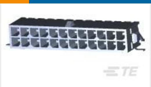
TE Part # 5-794629-4 24P MICRO MNL ASSY,R/A,SMT,LF
