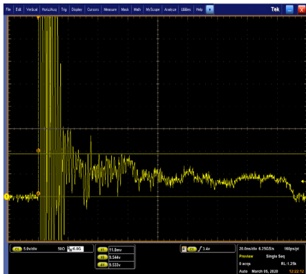
8/20μs Pulse Waveform
