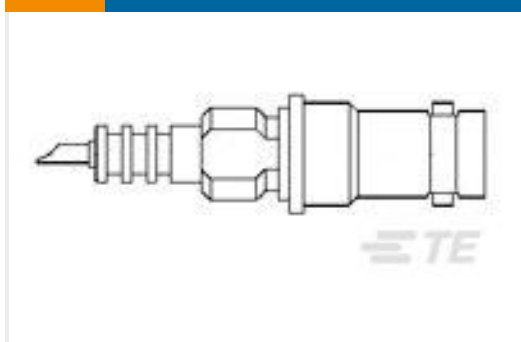
TE Part # 51494-2 STD HIGH VOLTAGE BLKHD RECEPT
