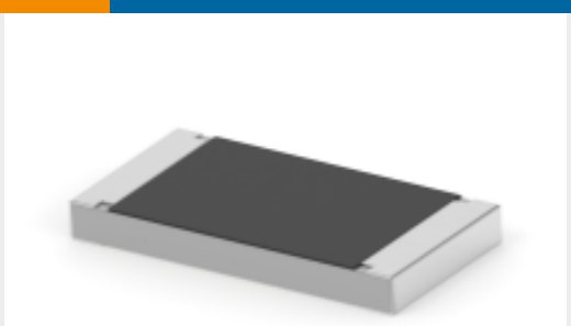
TE Part # 1-2176348-7 CRGCQ 2010 470R 5%
