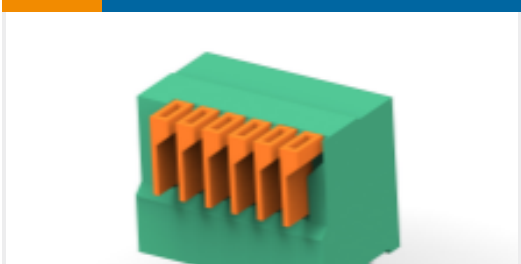
TE Part # 1-2834015-6 6POS 2.54MM TES CONN.
