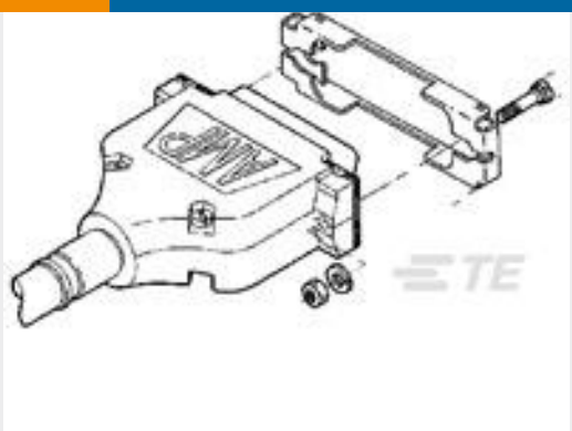
TE Part # 5745583-1 UNIV SLIDLTCH KIT SZ 2
