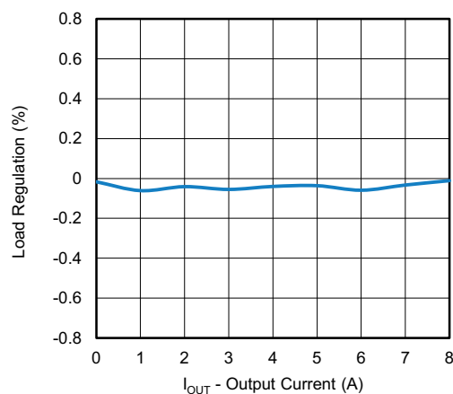
Fig. 44 - Load Regulation
