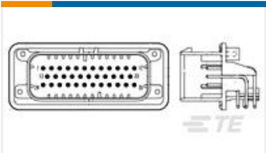
TE Part # 776163-2 35POS, PIN DIA 1.3, HDR ASSY, 90DEG, COD 2
