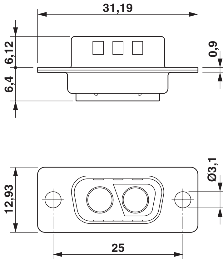
Dimensional drawing
