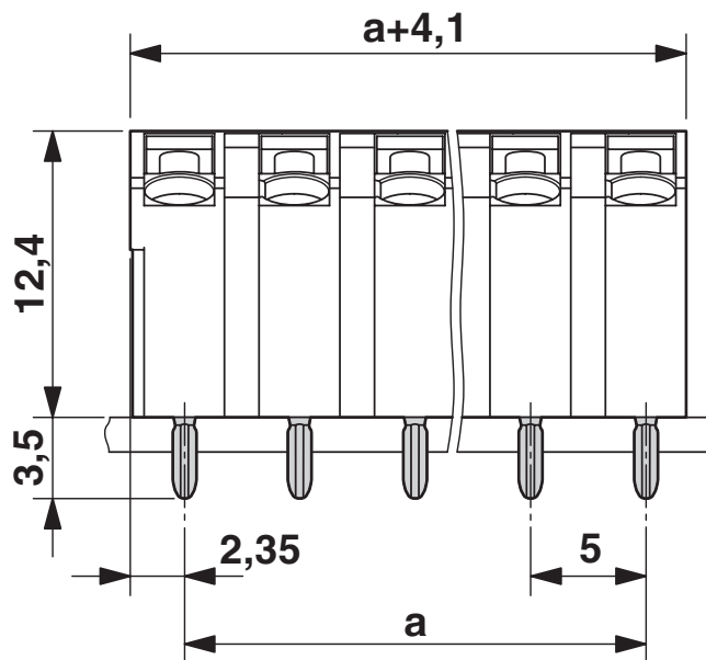
Dimensional drawing
