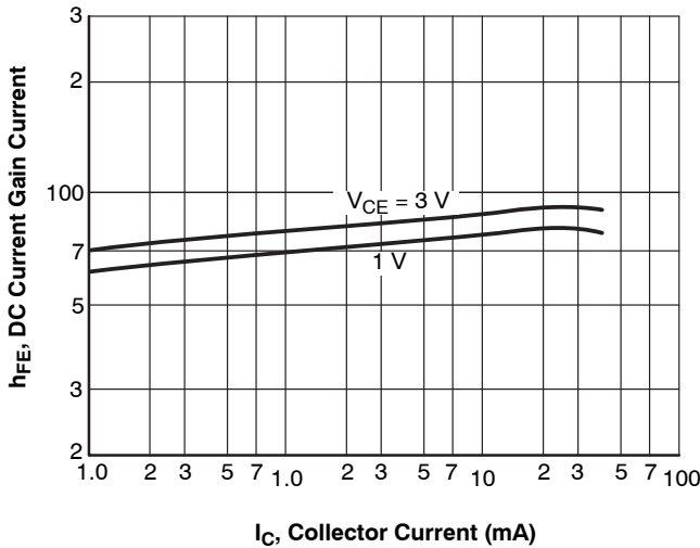
Figure 3. h_{FE} - I_C
