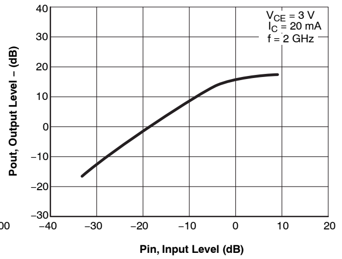
Figure 8. P_{out} - P_{in}
