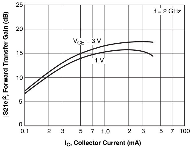
Figure 5. |S_{21e}|^2 - I_C
