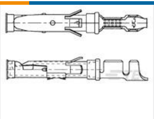
TE Part # 163088-2 LOOSE PC SOCKET TYPEIII+ CONTACT SIZE16
