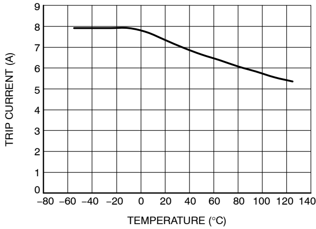
Figure 21. OCP Trip Current vs. Temperature (OCP = 32 k \Omega )
