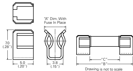
111 505 Device Dimensions
