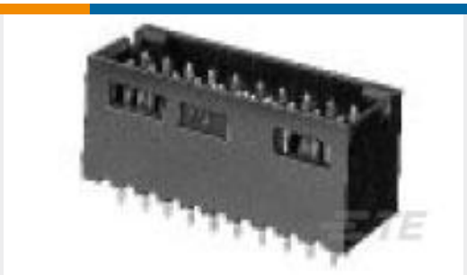
TE Part # 5-87589-4 16 MODII HDR DRST SHRDR .100CL
