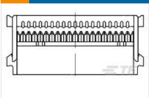
TE Part # 1-1658526-8 609-3430LF FEM SOCKET,LEAD FREE
