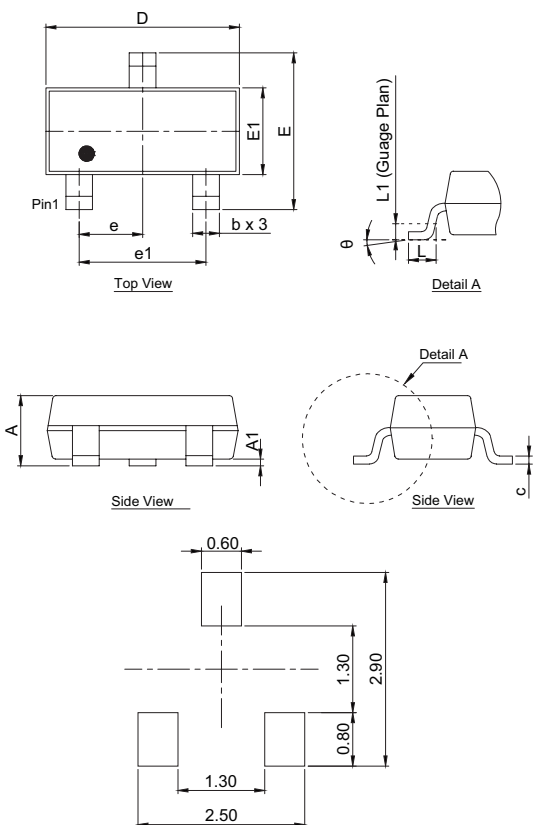
Recommended soldering pad layout (unit :mm)
