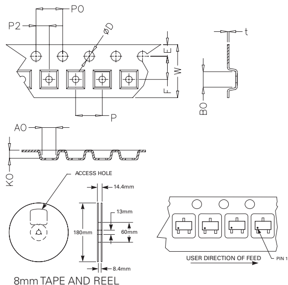
8mm TAPE AND REEL
