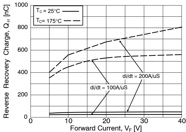
Figure 18. Stored Charge
