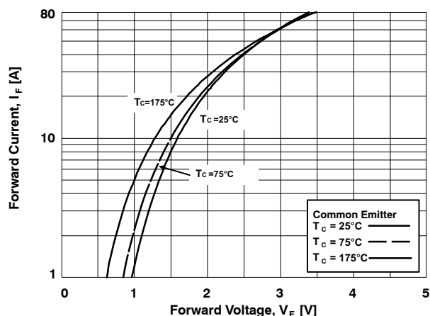
Figure 15. Forward Characteristics
