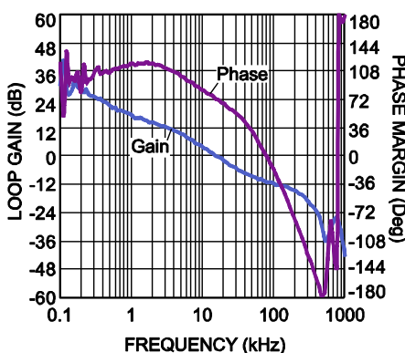
Bode Plot V_{IN}=6V , I_{OUT}=4A
