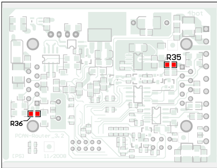
Position of the solder fields for the supply of external devices (D-Sub connector R35 for CAN1, R36 for CAN2)
