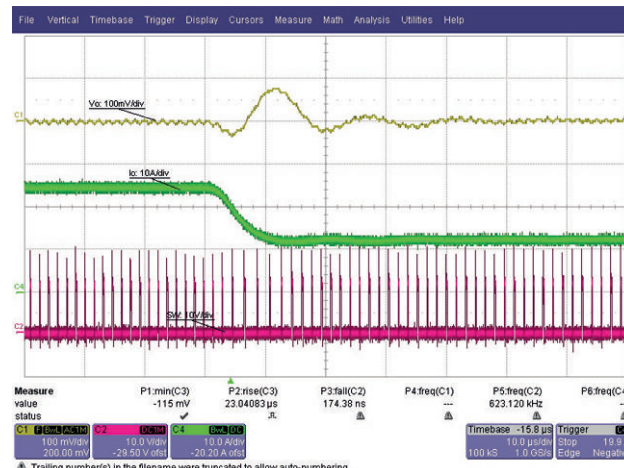
Fig. 30 - Load Release, 24 A to 12 A, 1 A/ \mu\text{s} , t = 10\text{ }\mu\text{s/div}
