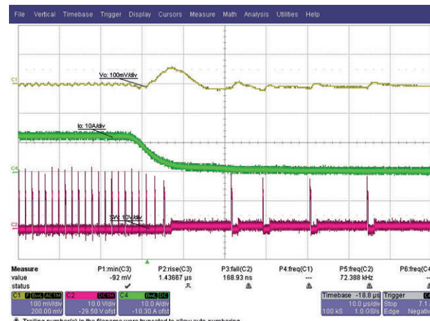
Fig. 31 - Load Release, 12 A to 0.1 A, 1 A/ \mu\text{s} , t = 20\text{ }\mu\text{s/div} Skip Mode Enabled
