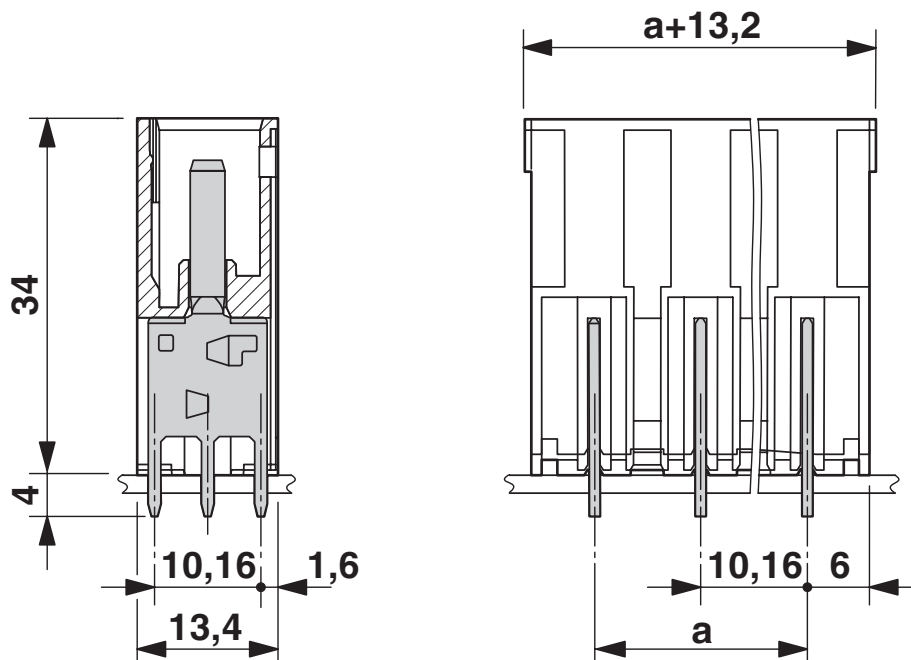
Dimensional drawing
