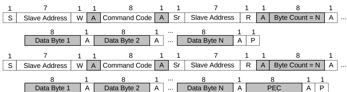
Figure 12: PMBus Message Format
