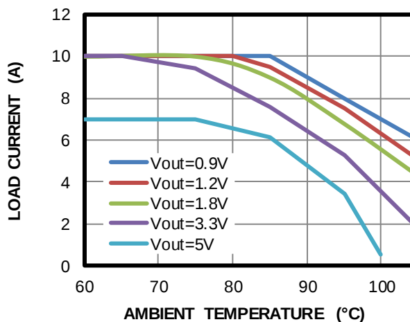
Thermal Derating
